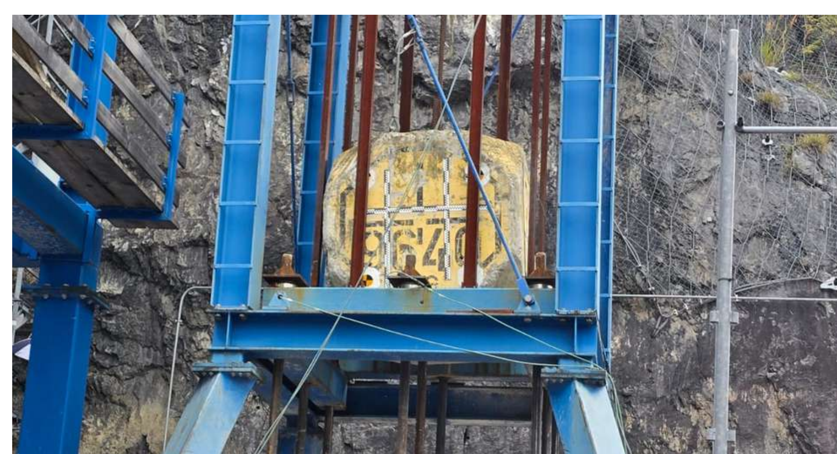
Geobrugg – Dynamic testing of tunnel support systems at the Walenstadt test facility
