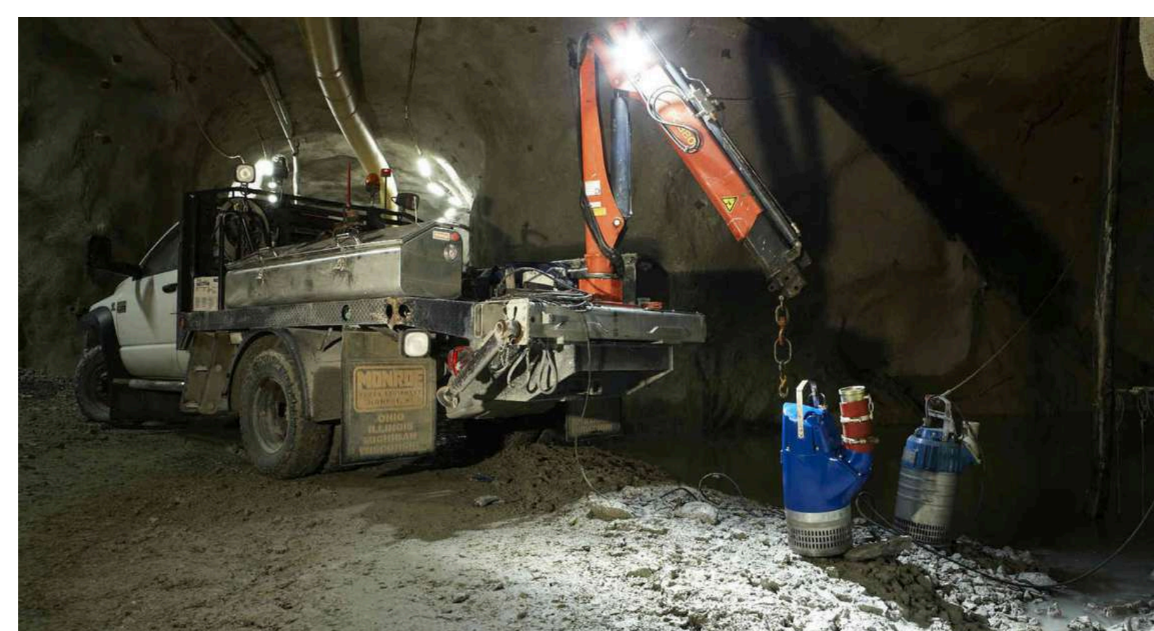
Sulzer - Dewatering pumps optimizing operations at Boliden Garpenberg mine, Sweden
